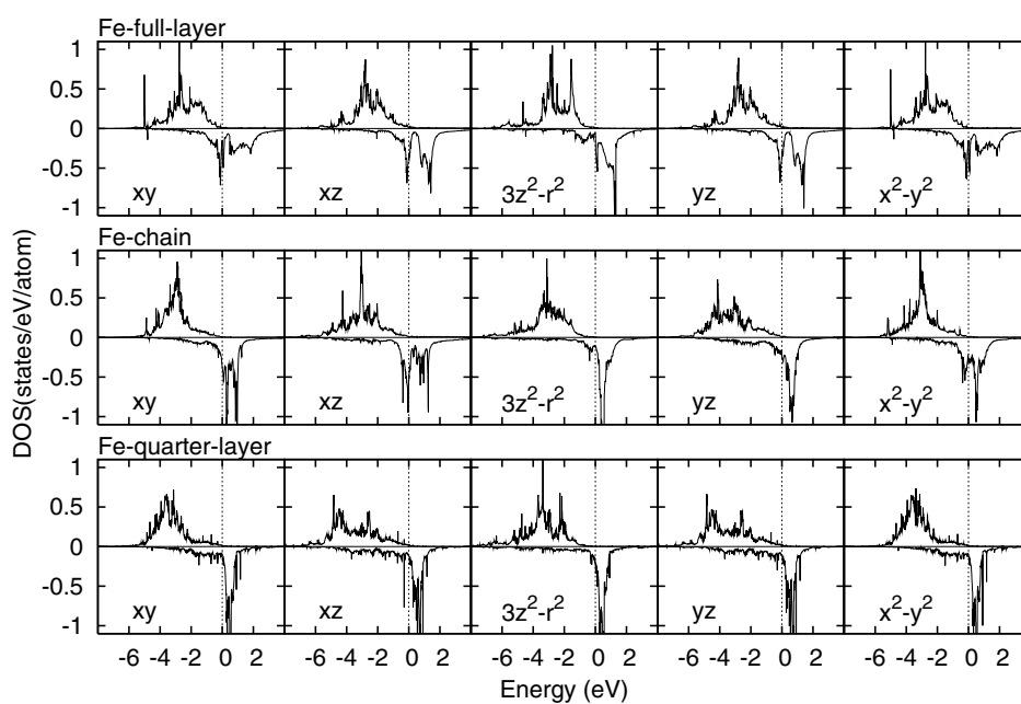
Figure 2. Partial densities of states projected to the components of d_{xy} , d_{xz} , d_{3z^2-r^2} , d_{yz} , d_{x^2-y^2} in an Fe atom for the Fe-full-layer (top), Fe-chain (middle) and Fe-quarter-layer (bottom) on the Pt(111) surface.
